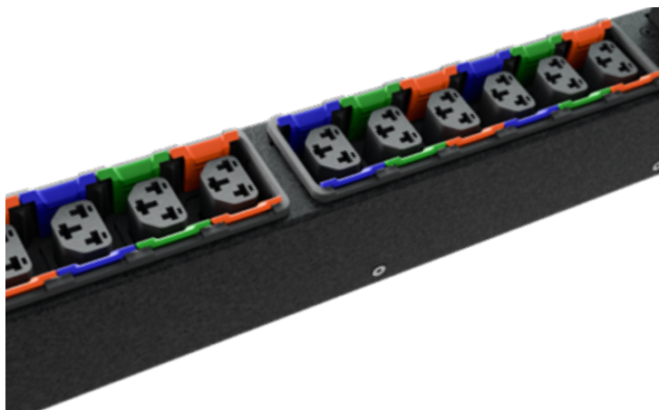
Receptacles on the Vertiv rPDUs are color coded by phase to simplify load balancing.
