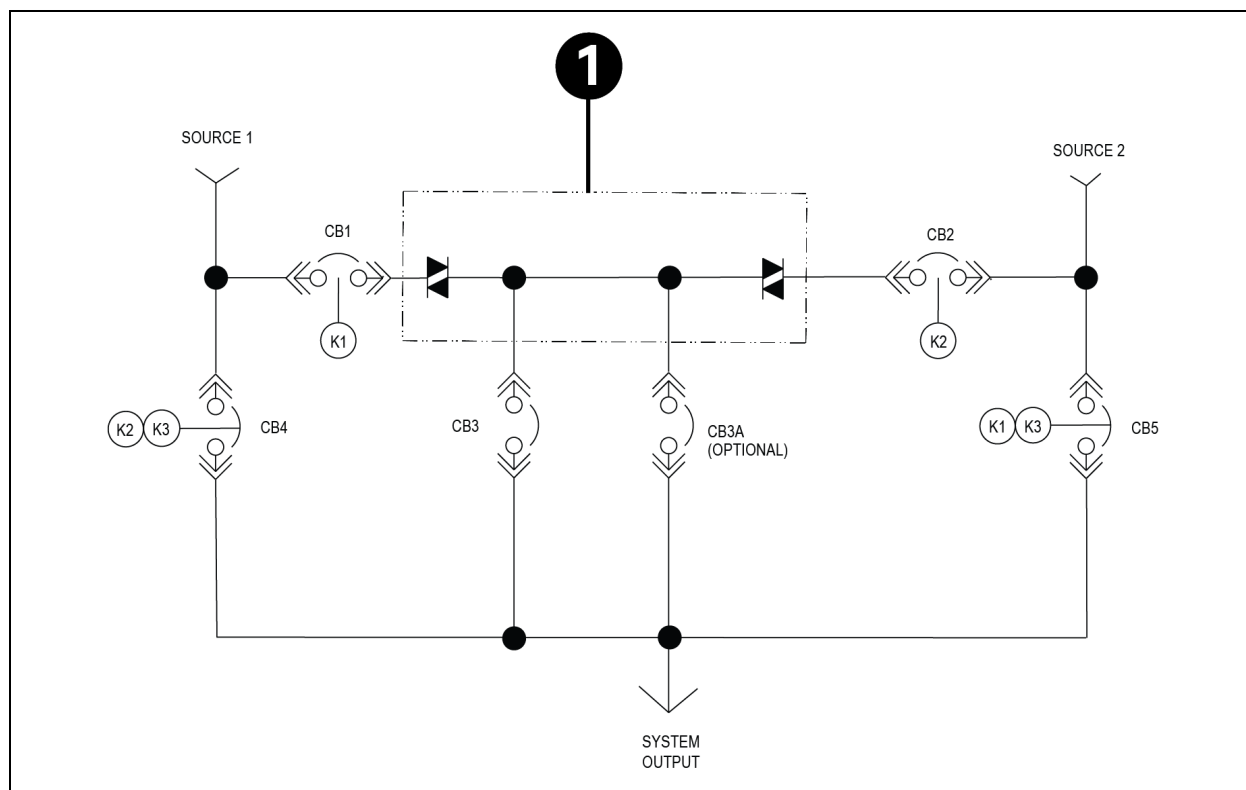
Figure 5.1 Typical Static Transfer Switch One-Line Diagram
