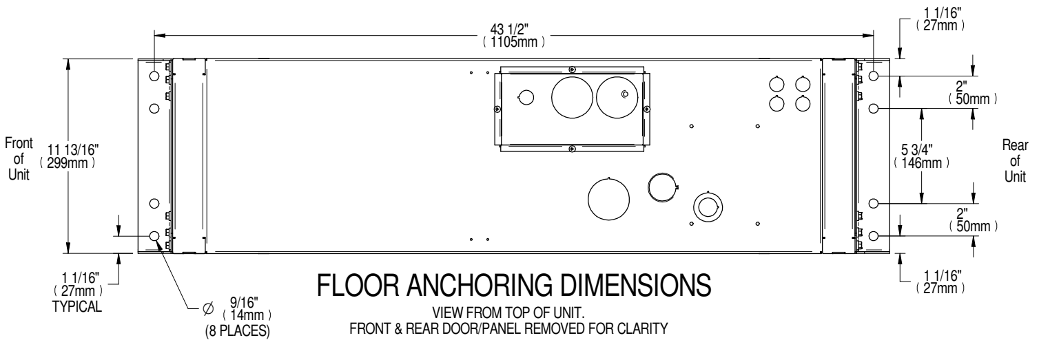
ANCHORAGE DETAIL 4
