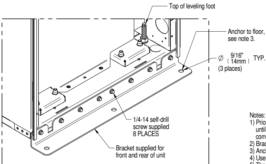
DETAIL A
