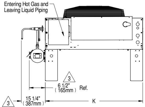
Front View (Liebert® Lee-Temp Shown)
