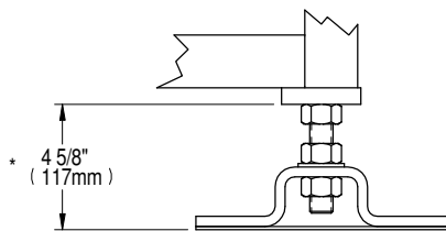
FOOT DETAIL
