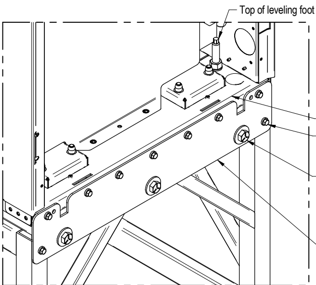
DETAIL A
