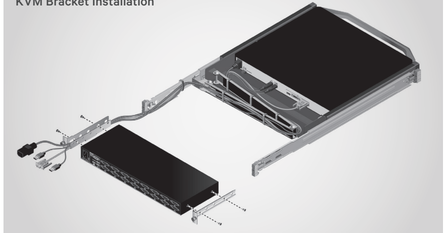
KVM Bracket Installation
