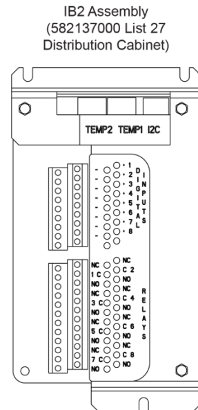
Figure 5 External Alarm, Reference, Monitoring, and Control Connections, IB2 (Controller Interface Board)
