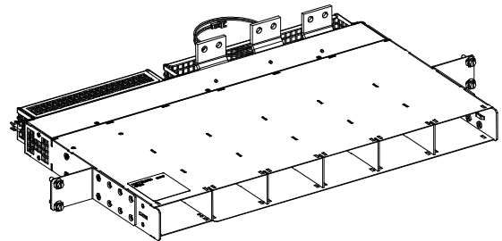
P/N 557352 Rail Mounting Kit
