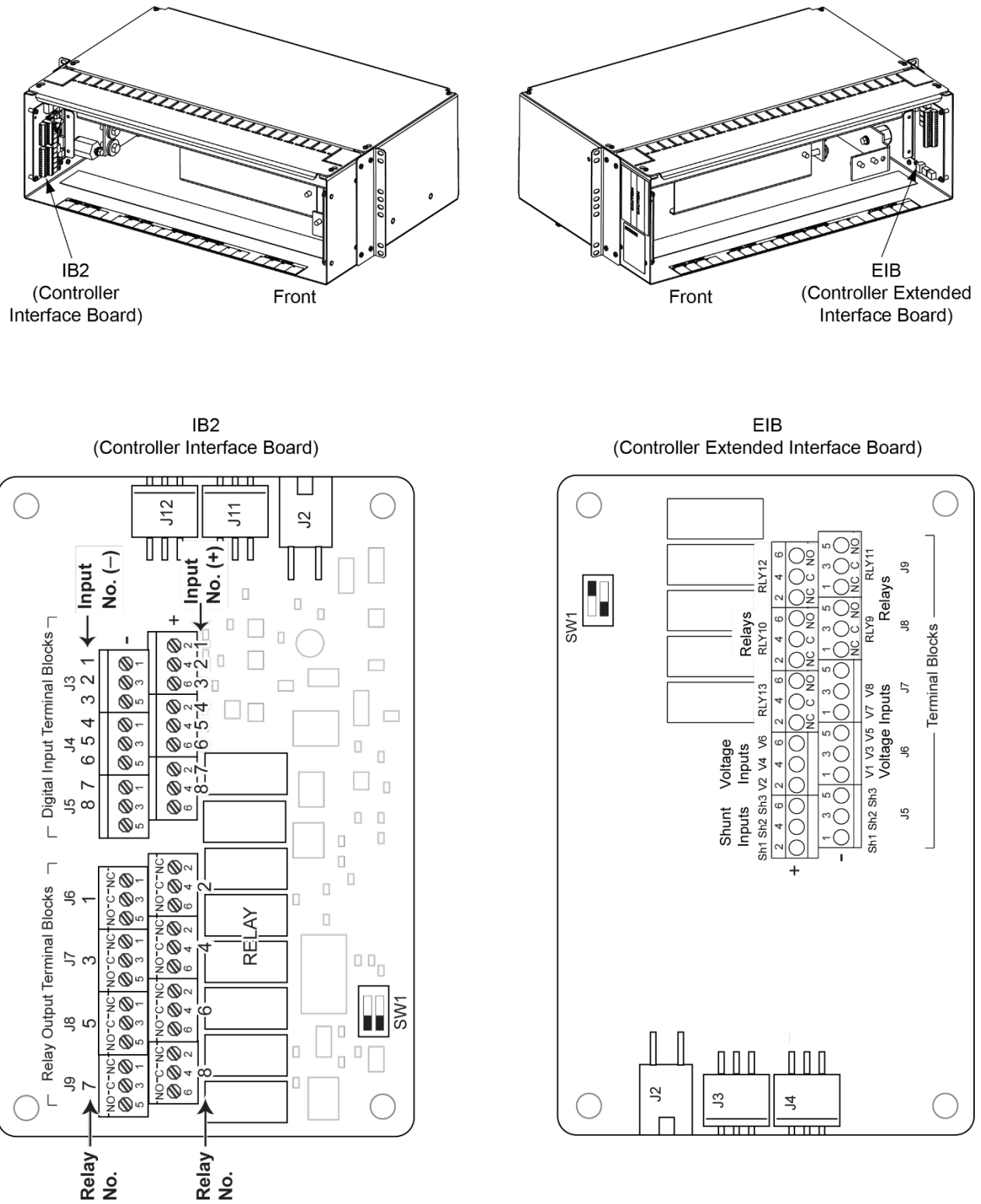
Figure 2 External Alarm, Reference, Monitoring, and Control Connections Locations in a 582137000 List 7 Distribution Cabinet
